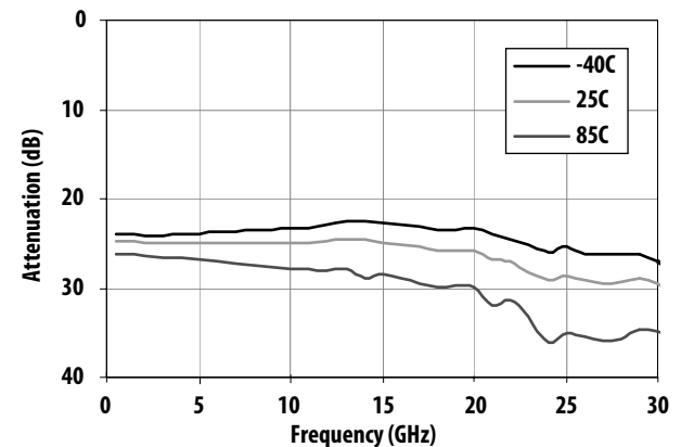
Figure 12. Attenuation vs Frequency (Max Attenuation)
