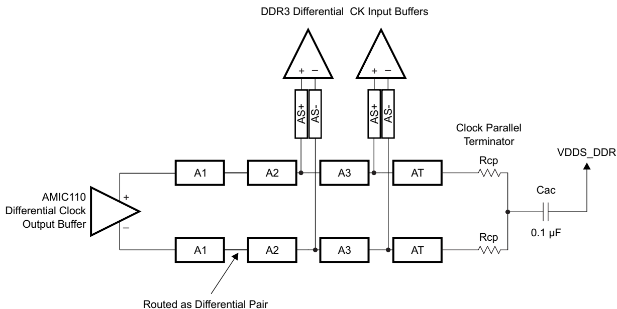
Figure 7-38. CK Topology for Two DDR3 Devices
