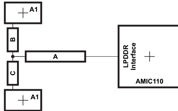
Figure 7-22. CK and ADDR_CTRL Routing and Topology
