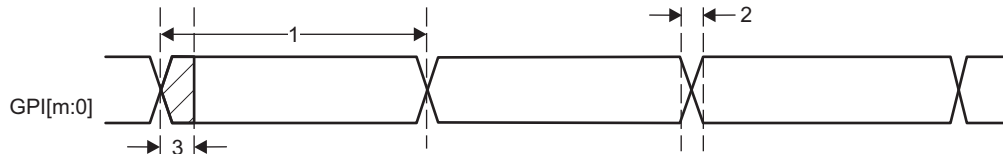
Figure 7-67. PRU-ICSS PRU Direct Input Timing
