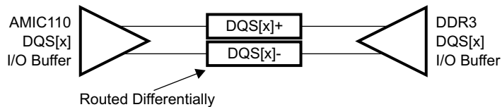
Figure 7-48. DQS[x] Topology
