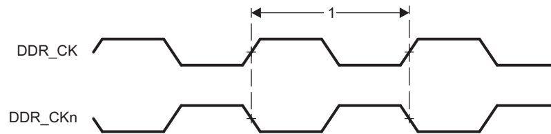
Figure 7-24. DDR2 Memory Interface Clock Timing
