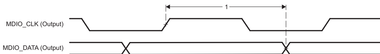
Figure 7-79. PRU-ICSS MDIO_DATA Timing – Output Mode
