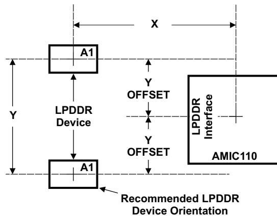
Figure 7-20. AMIC110 Device and LPDDR Device Placement
