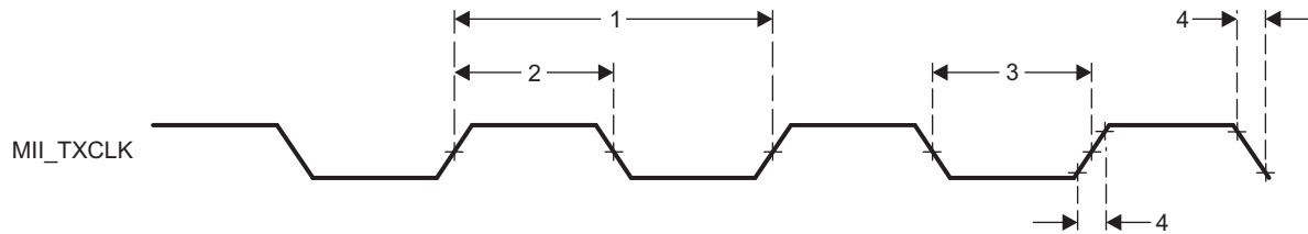
Figure 7-81. PRU-ICSS MII_TXCLK Timing
