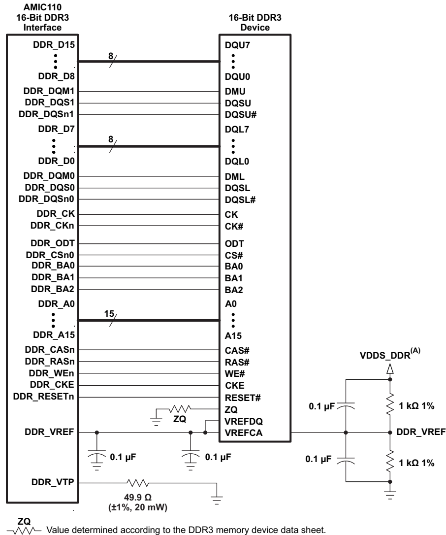
Figure 7-34. 16-Bit DDR3 Interface Using One 16-Bit DDR3 Device without V_{TT} Termination
