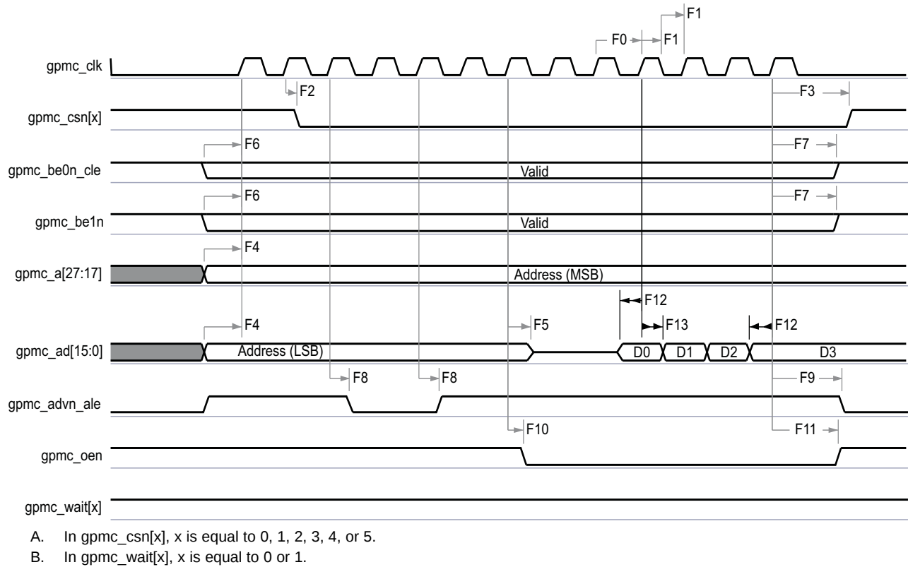
Figure 7-6. GPMC and Multiplexed NOR Flash—Synchronous Burst Read
