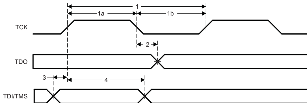
Figure 7-56. JTAG Timing
