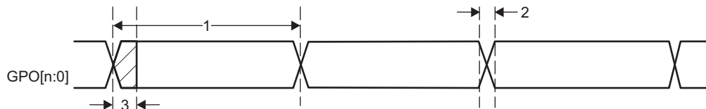
Figure 7-68. PRU-ICSS PRU Direct Output Timing
