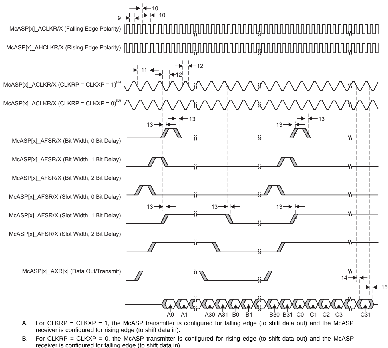
Figure 7-58. McASP Output Timing
