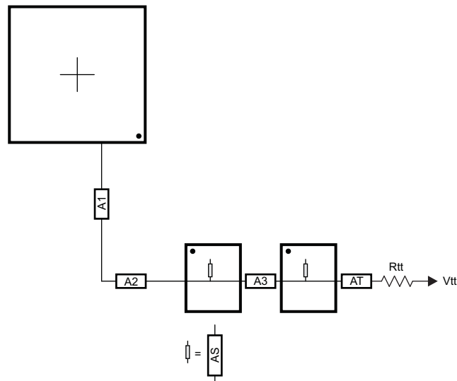
Figure 7-41. ADDR_CTRL Routing for Two Single-Sided DDR3 Devices
