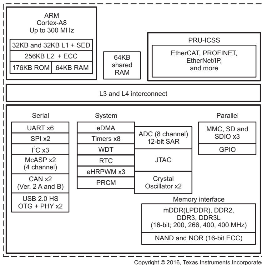
Figure 1-1. AMIC110 Functional Block Diagram
