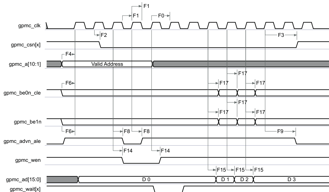
Figure 7-5. GPMC and NOR Flash—Synchronous Burst Write—(GpmcFCLKDivider > 0)
