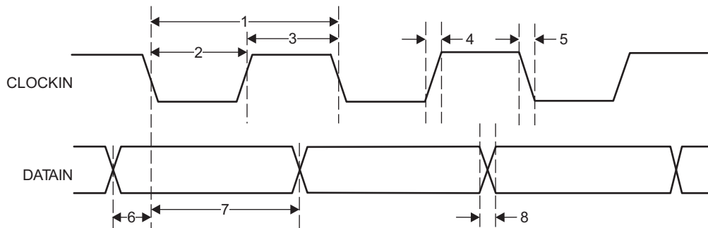
Figure 7-70. PRU-ICSS PRU Parallel Capture Timing - Falling Edge Mode
