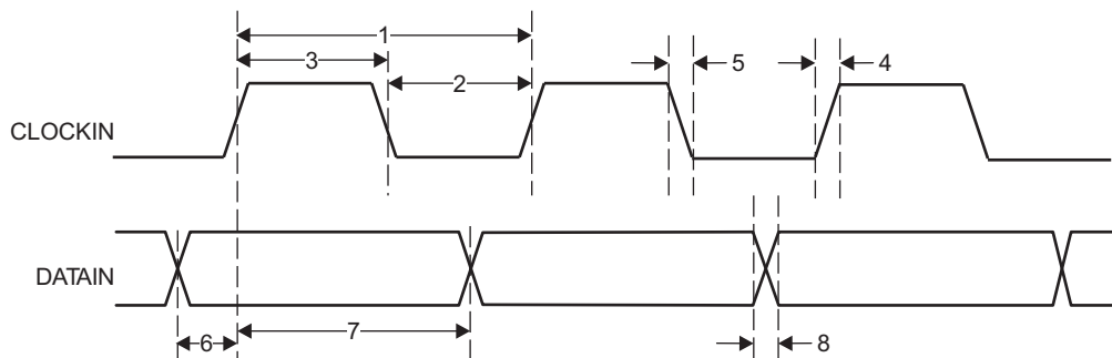
Figure 7-69. PRU-ICSS PRU Parallel Capture Timing - Rising Edge Mode
