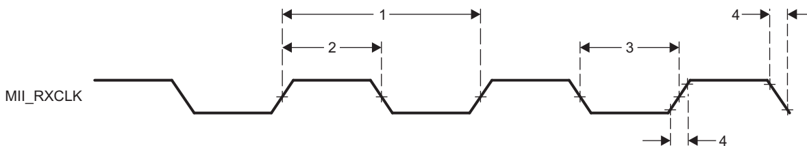
Figure 7-80. PRU-ICSS MII_RXCLK Timing
