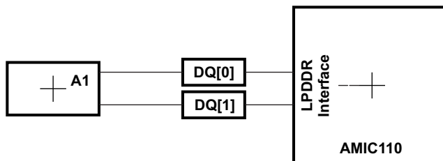
Figure 7-23. DQS[x] and DQ[x] Routing and Topology
