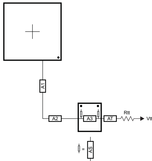
Figure 7-43. ADDR_CTRL Routing for Two Mirrored DDR3 Devices
