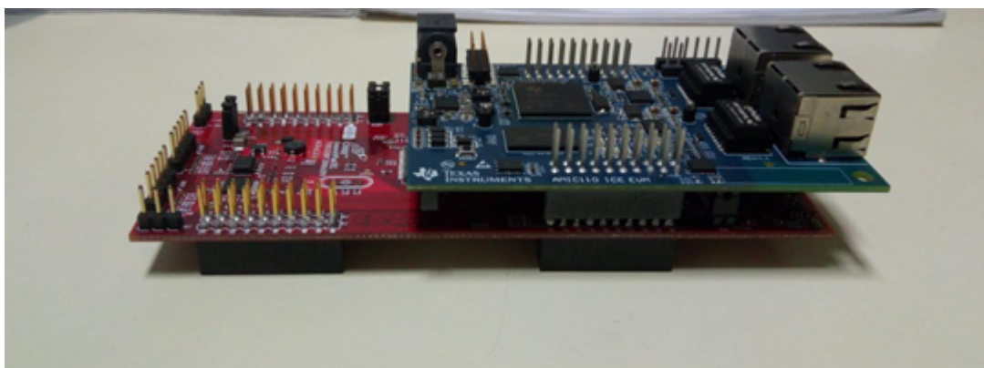
Figure 24. Connected Devices
