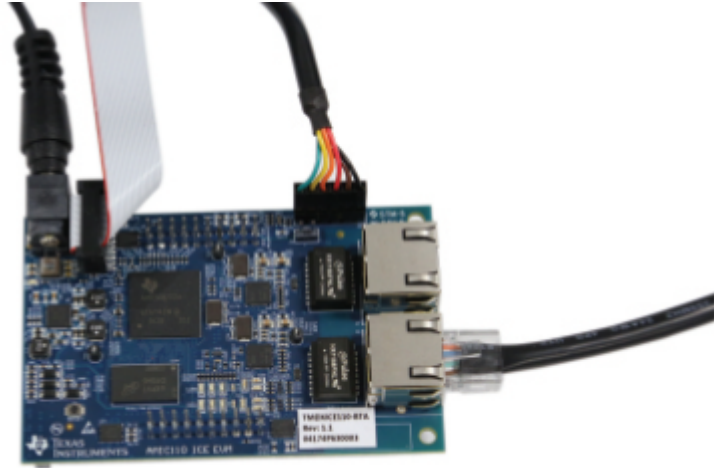
Figure 4. AMIC110 ICE Power Supply Connection
