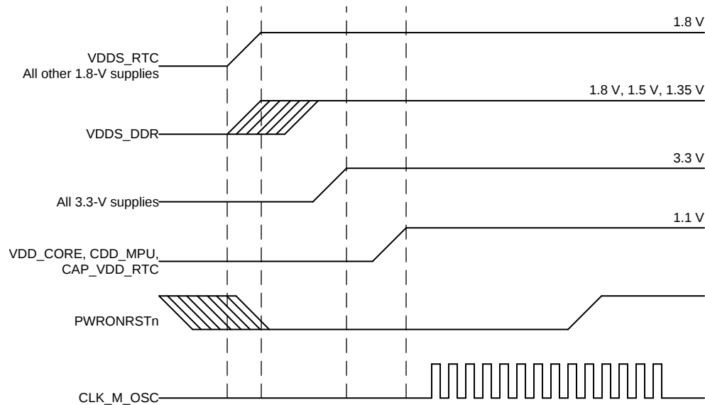
Figure 17. Power-Up Sequence
