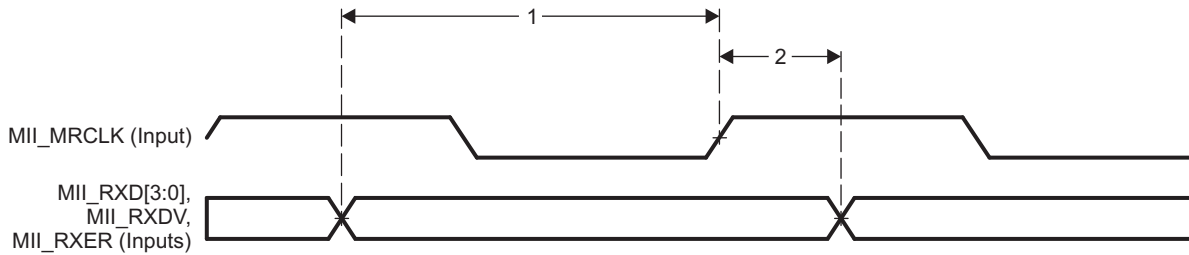
Figure 7-96. PRU-ICSS MII_RXD[3:0], MII_RXDV, and MII_RXER Timing
