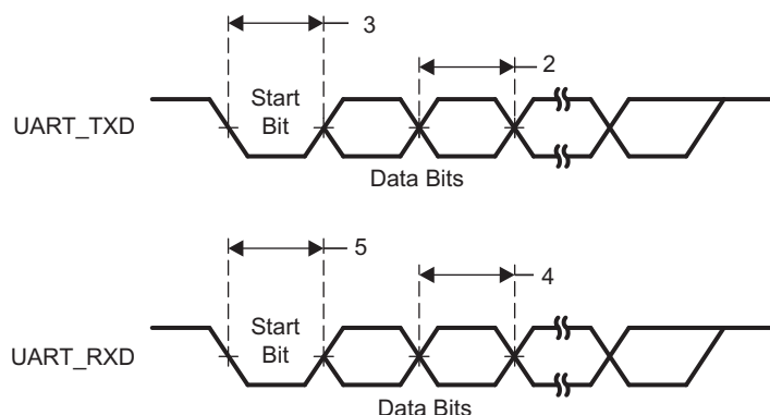
Figure 7-98. PRU-ICSS UART Timing
