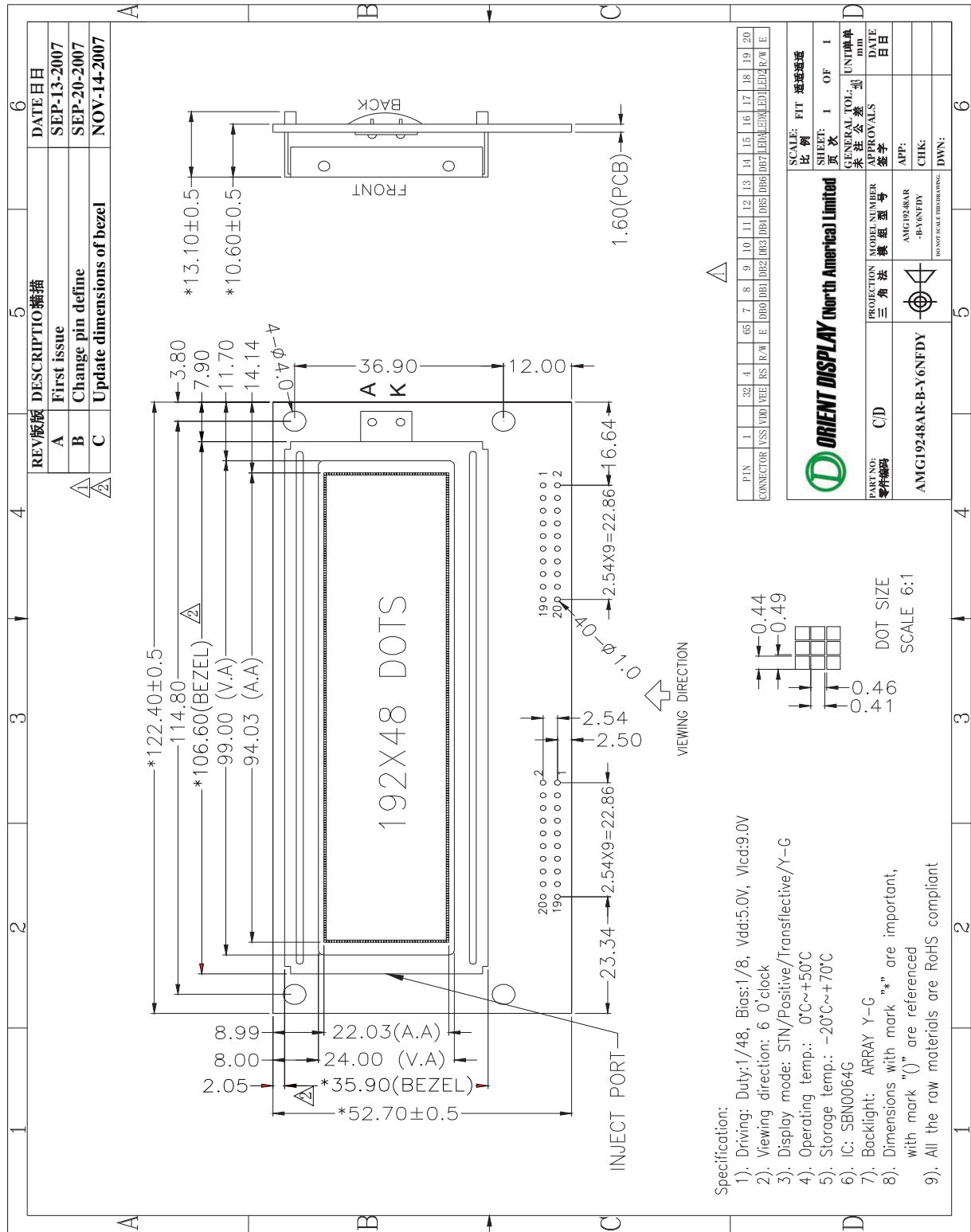
Figure 1. Dimensional outline
