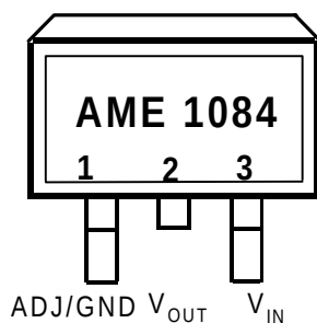
TO-263-2 Front View
