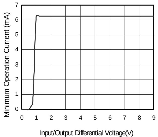
Minimum Operation Current vs Input/Output Differential Voltage
