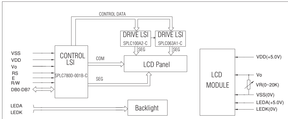
Figure 2. Block diagram
