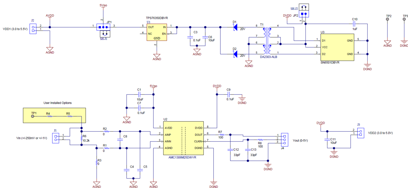
Figure 6. AMC1306EVM Schematic
