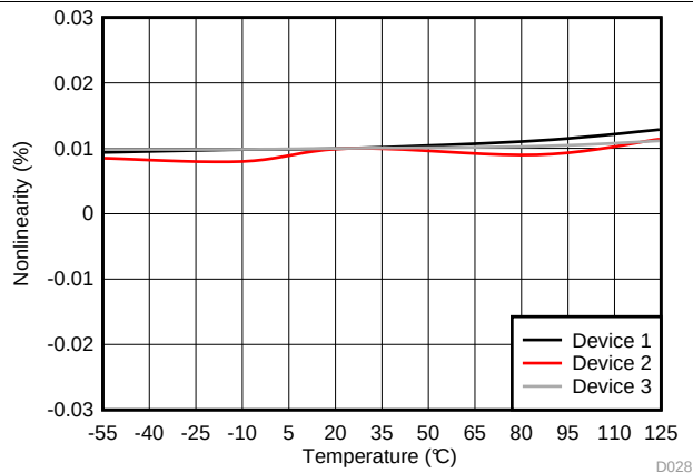
Figure 29. Nonlinearity vs Temperature
