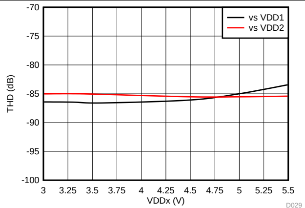
Figure 30. Total Harmonic Distortion vs Supply Voltage
