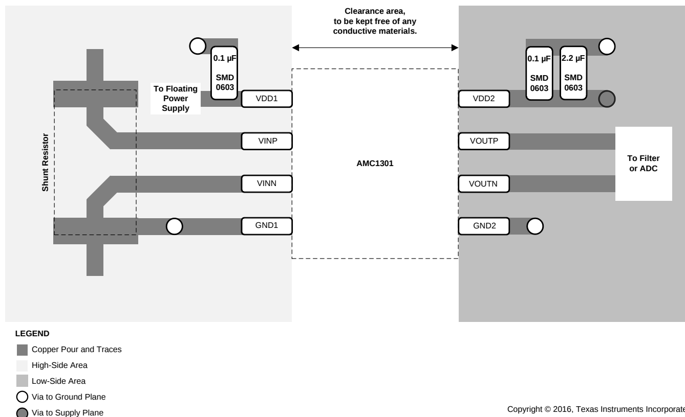
Figure 55. Recommended Layout of the AMC1301 Device
