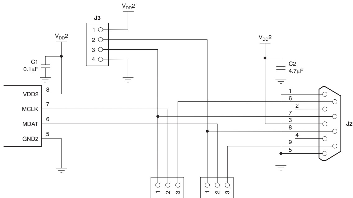
Figure 2. Power and Digital Outputs
