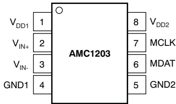
DUB or PSA PACKAGE SOP-8 Gull-Wing or SOP-8 (TOP VIEW)
