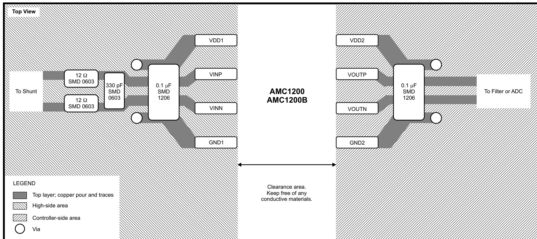
Figure 33. Layout Recommendation
