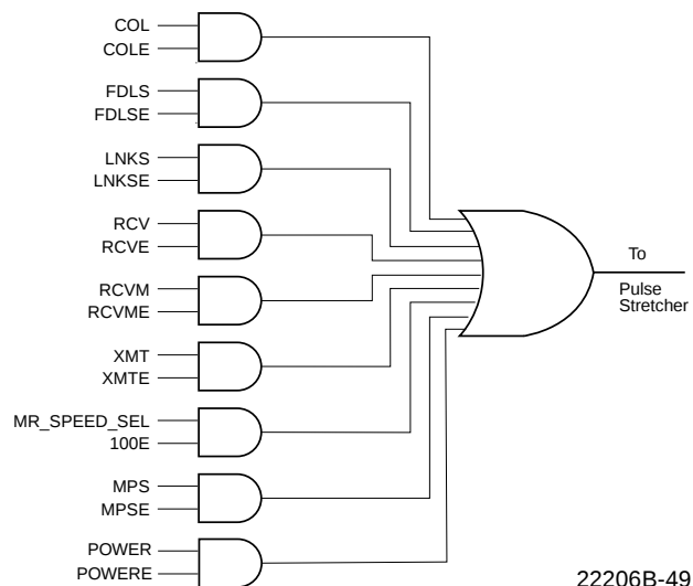
Figure 45. LED Control Logic
