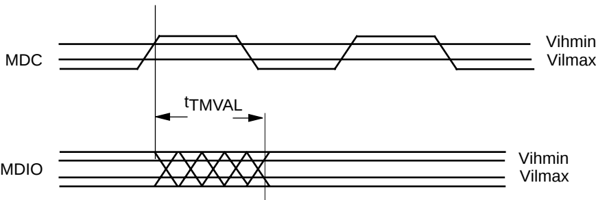
Figure 70. Management Data Output Valid Delay Timing
