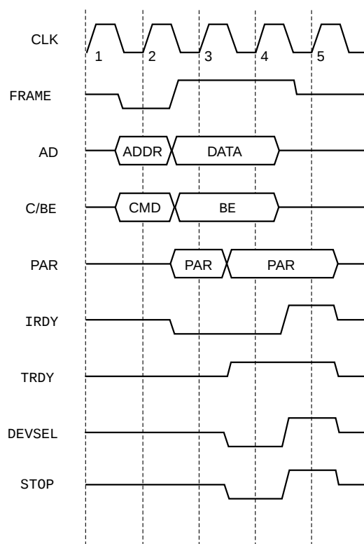
Figure 8. Disconnect of Slave Cycle When Busy
