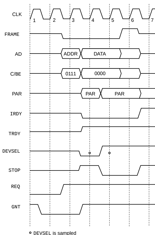
Figure 20. Target Abort
