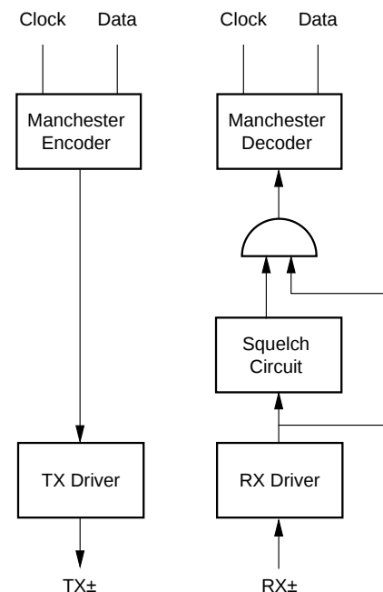
Figure 50. 10BASE-T Transmit and Receive Data Paths
