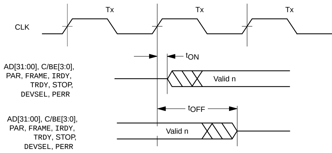
Figure 61. Output Tri-State Delay Timing
