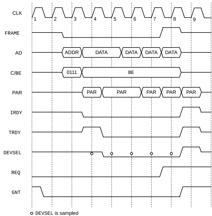
Figure 17. Burst Write Transfer (EXTREQ = 1)
