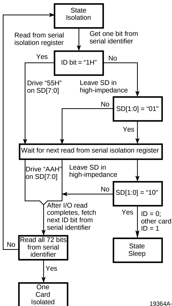
Plug and Play ISA Card Isolation Algorithm
