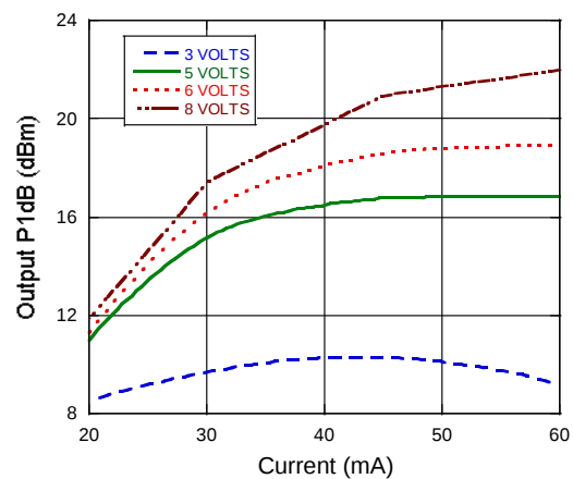
Output P1 dB vs. Current, F = 1785 MHz
