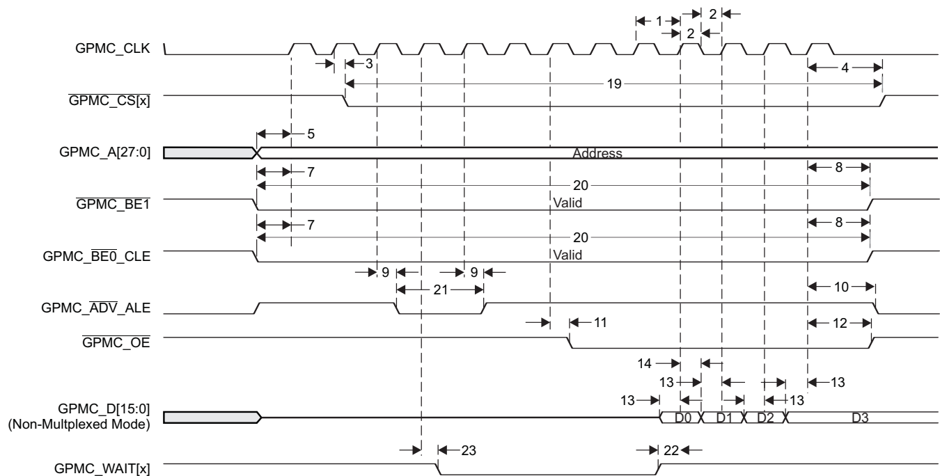
Figure 8-22. GPMC Non-Multiplexed NOR Flash - 14x16-bit Synchronous Burst Read (GPMCCLKDIVIDER = 0)
