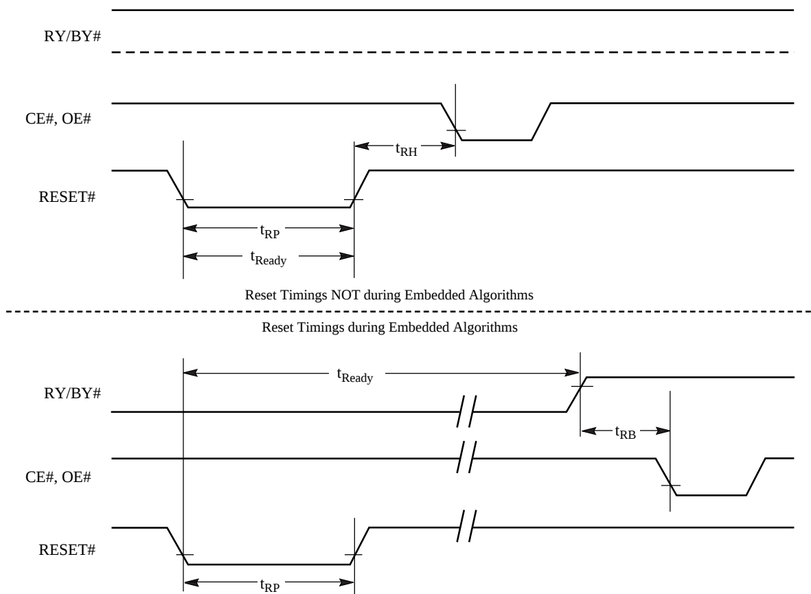
Figure 1. RESET# Timings
