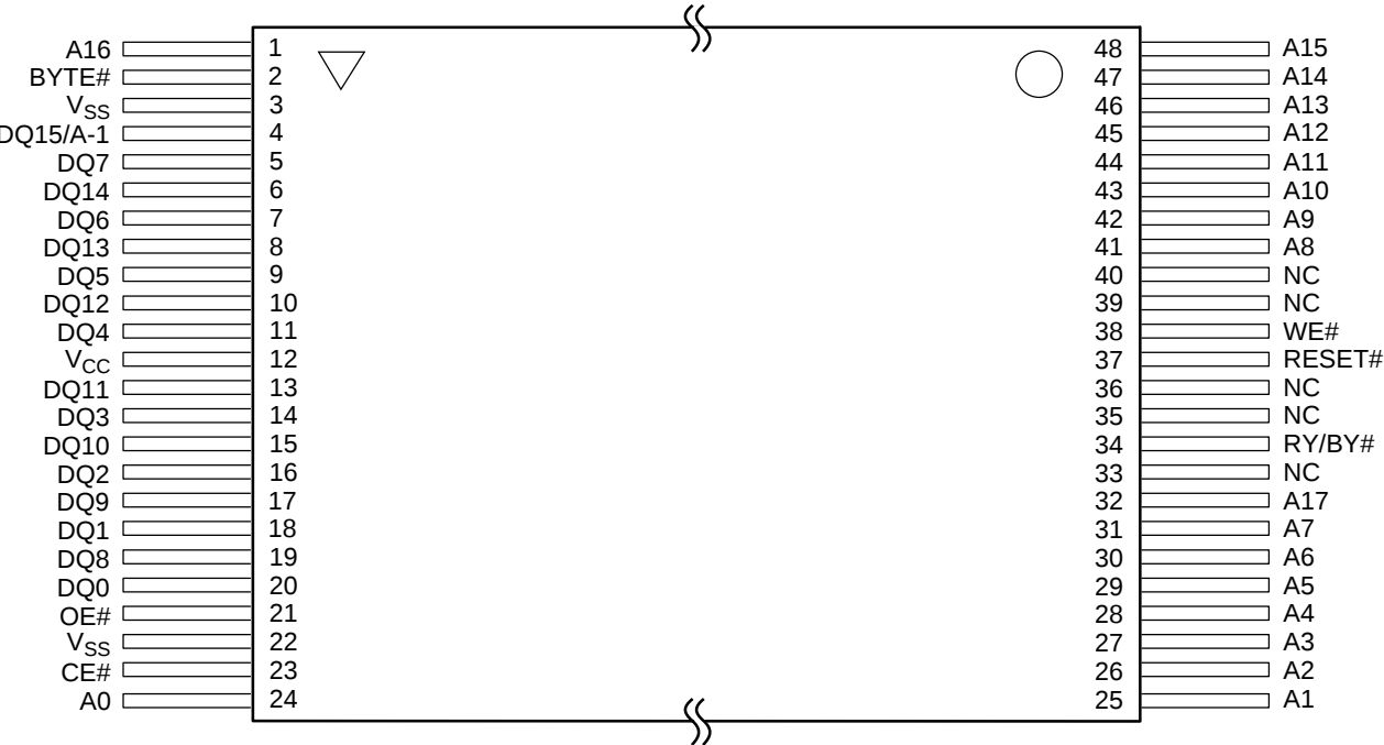
48-Pin TSOP—Reverse Pinout
