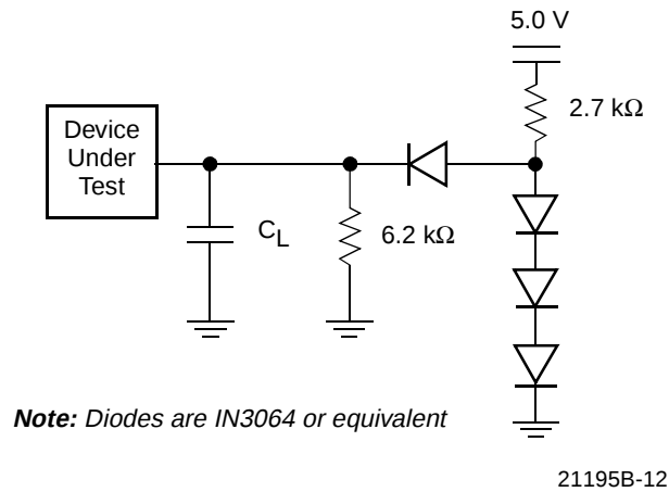
Figure 8. Test Setup
