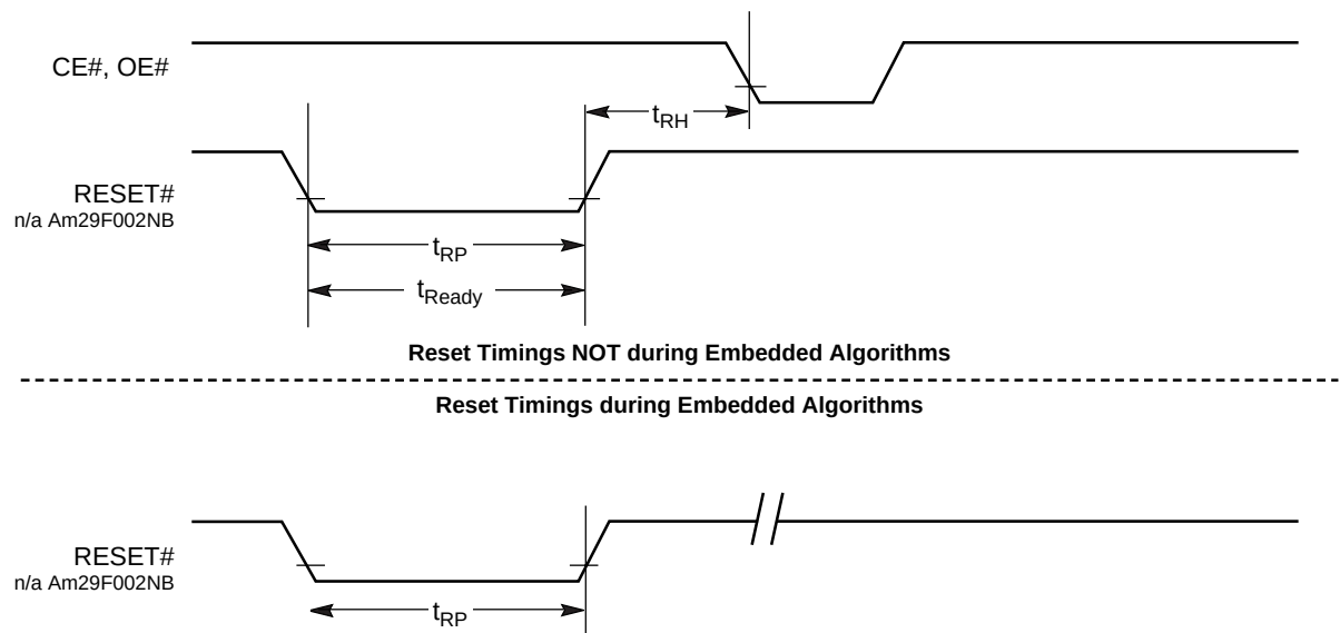
Figure 10. RESET# Timings
