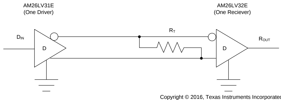
Figure 19. Differential Terminated Configuration
