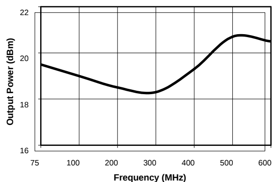
1 dB Compression
