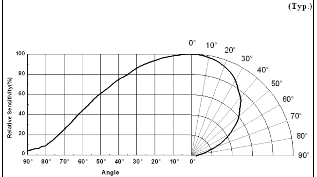
Fig 12 Relative Sensitivity vs. Angle
