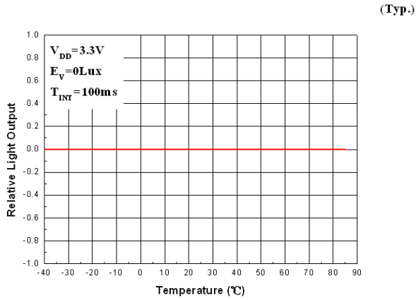
Fig 9 Light Output vs. Temperature
