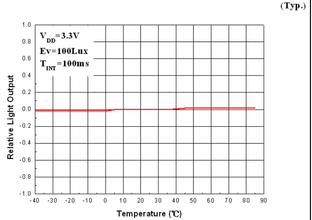
Fig 10 Light Output vs. Temperature
