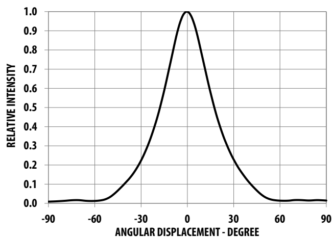
Figure 10: Radiation Pattern
