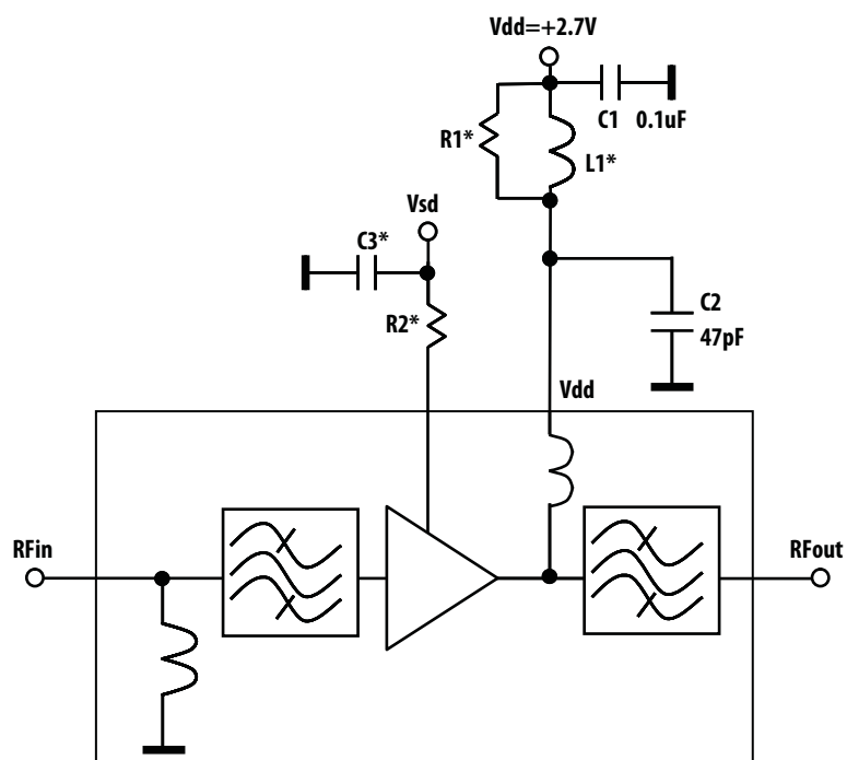
Figure 2. Application Circuit
