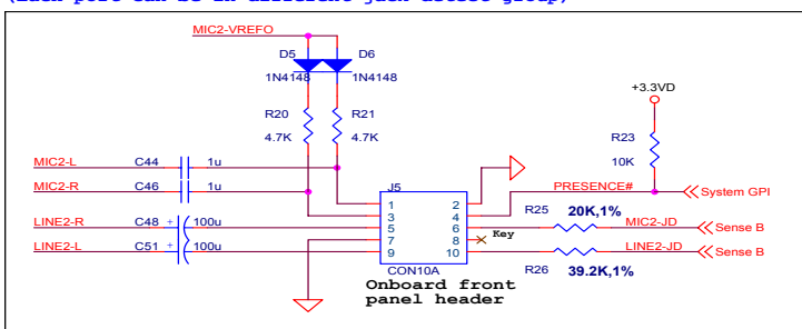
Figure 19. Onboard Front Panel Header Connection
