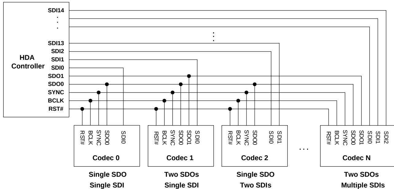
Figure 7. Signaling Topology
