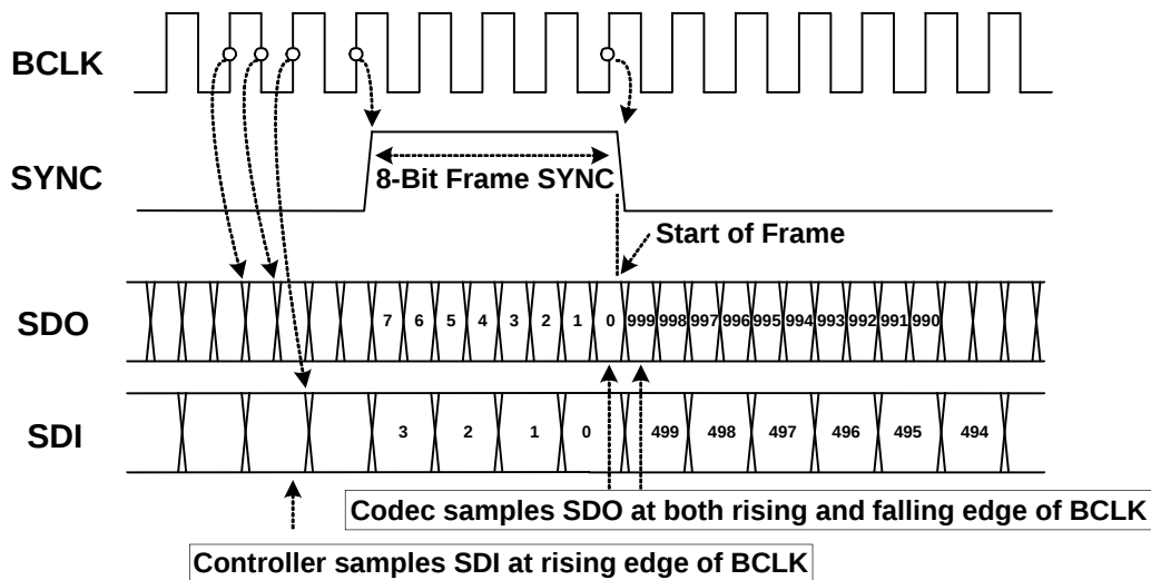
Figure 6. Bit Timing
