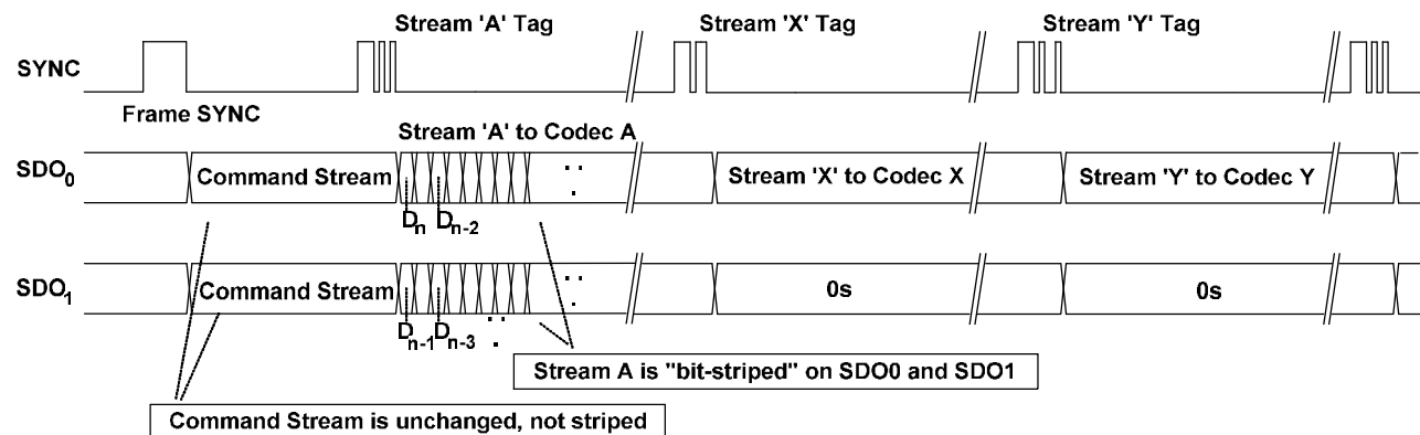
Figure 10. Striped Stream on Multiple SDOs
