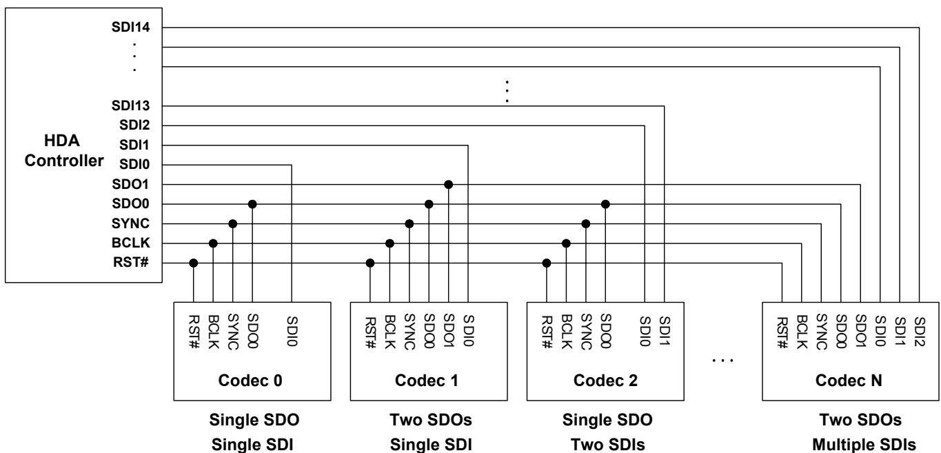
Figure 5. Signaling Topology
