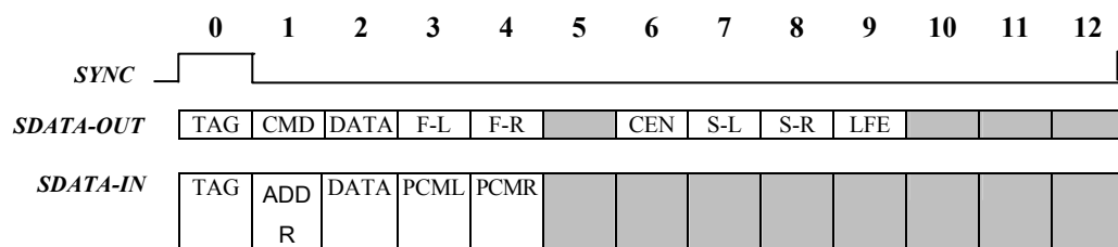
Fig7.2-2 Default ALC650 slot arrangement – CODEC ID = 00
