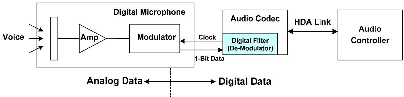
Figure 22. Digital Microphone Implementation-1
