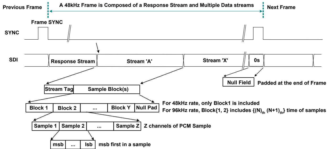
Figure 12. SDI Inbound Stream
