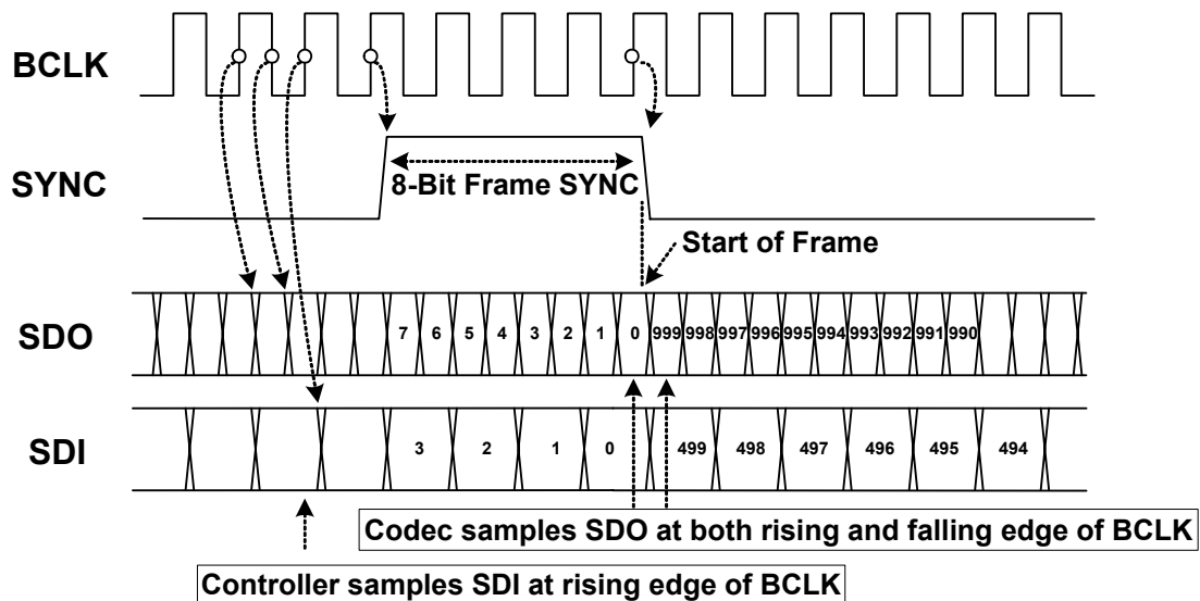
Figure 7. Bit Timing
