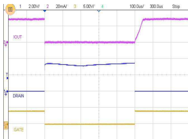
Figure 8 Minimum Off Pulse Width ( t_{OFF\_MIN} )
