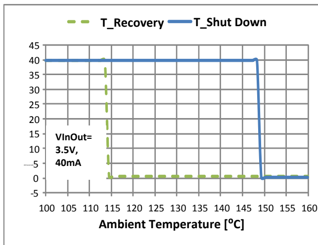
Figure 19 THSD of 40mA Current Option
