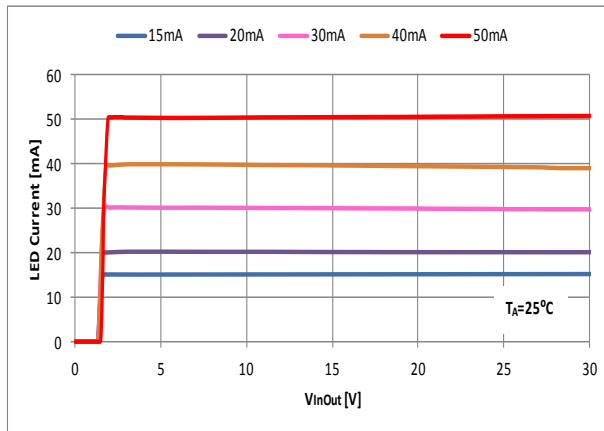
Figure 1. LED Current vs. VinOut
