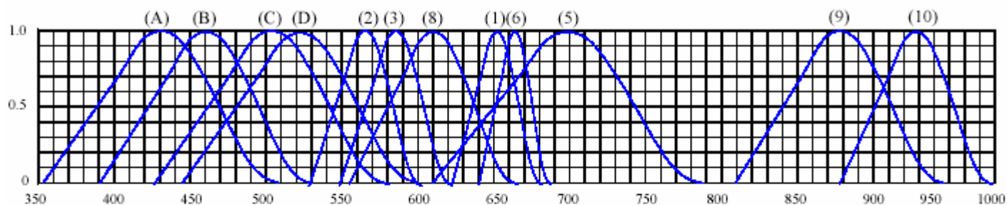
Wavelength(nm) RELATIVE INTENSITY VS. WAVELENGTH( \lambda_p )
