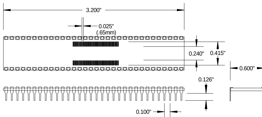
AK64D600-TSSOP.65 .65MM TSSOP TO 64 PIN DIP
