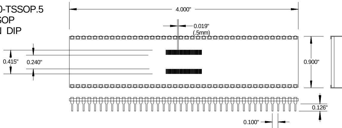
AK80D900-QFP.65mm QFP 0.65mm PITCH TO 80 PIN DIP
