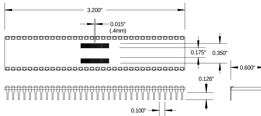
AK64D600-TSSOP.4 .4MM TSSOP TO 64 PIN DIP
