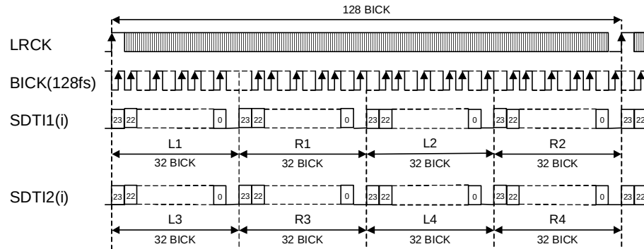
Figure 8. Mode 8 Timing
