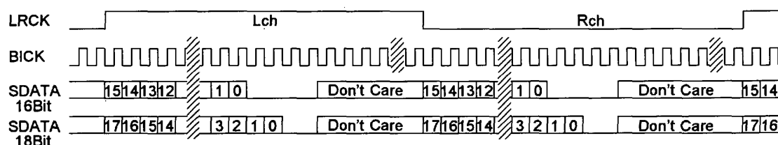
Figure 3 . Mode 2 Timing
