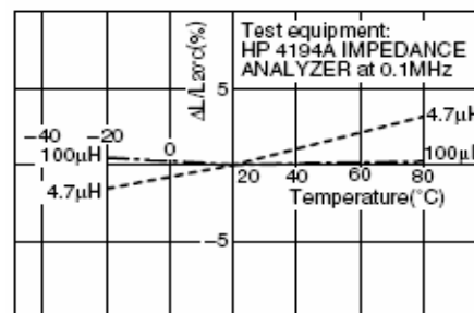
INDUCTANCE CHANGE vs. TEMPERATURE CHARACTERISTICS
