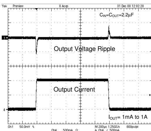
Fig.11 Load Transient Response at V_{IN}=2.3V , V_{OUT}=0.8V
