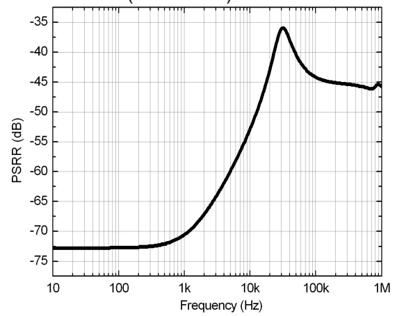
Fig. 14 PSRR Curve
