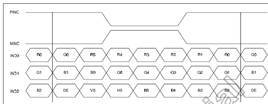
Figure 10.4: 6-bit LVDS input
