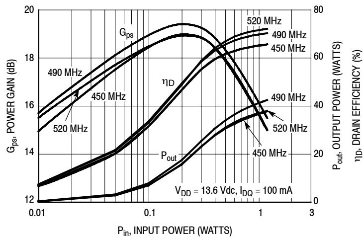
Figure 22. Power Gain, Output Power and Drain Efficiency versus Input Power and Frequency
