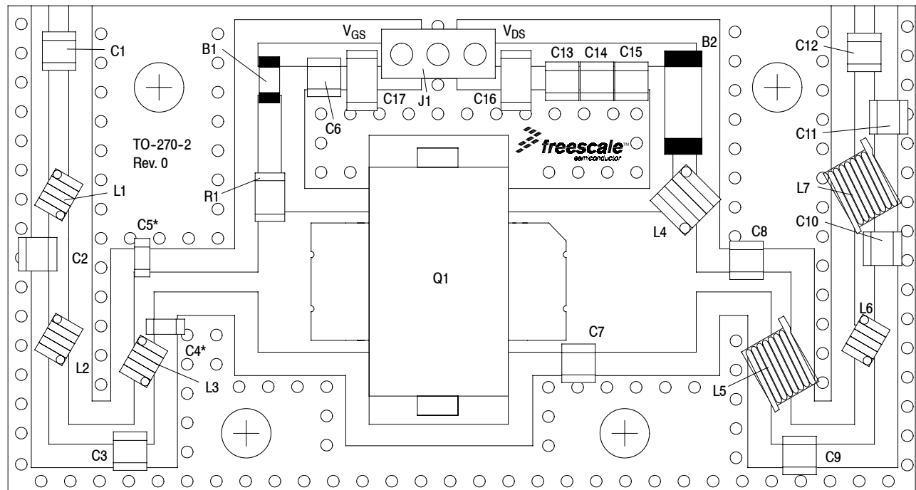
Figure 10. AFT05MS031NR1 UHF Wideband Reference Circuit Component Layout — 380-450 MHz
