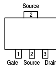
Figure 1. Pin Connections
