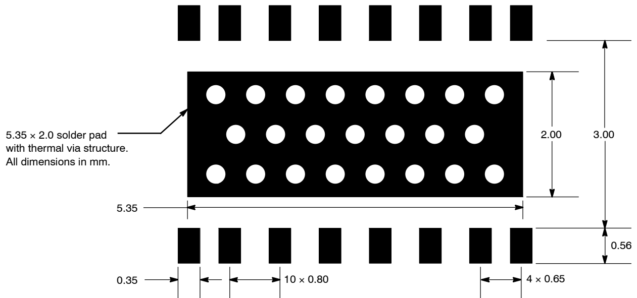
Figure 12. PCB Pad Layout for 16-Lead DFN 4 x 6
