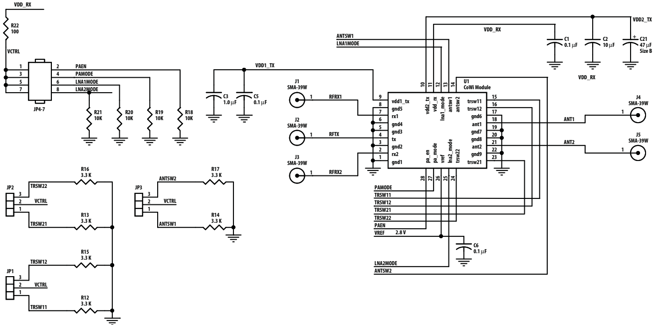
Figure 3. Demoboard Schematic
