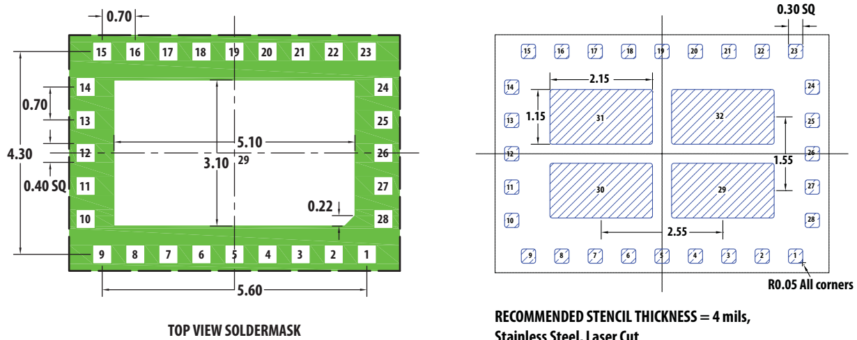
Figure 6. Recommended Soldermask
