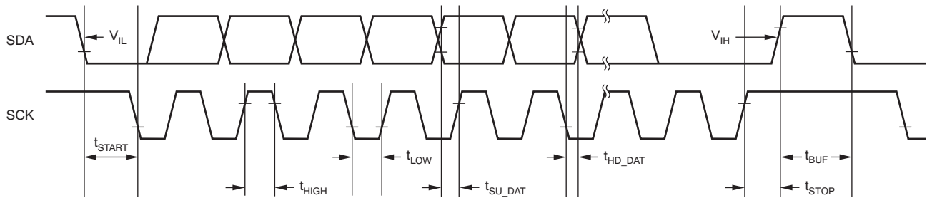
Figure 3. I 2 C Bus Interface Timing
