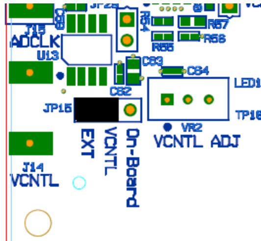
Figure 28. Vcntl
