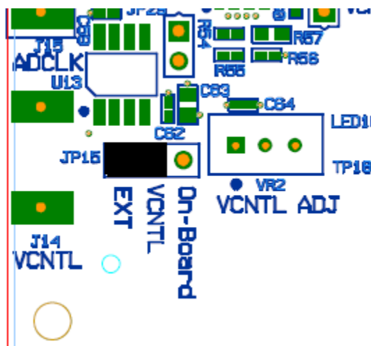
Figure 25. External Vcntl Configuration
