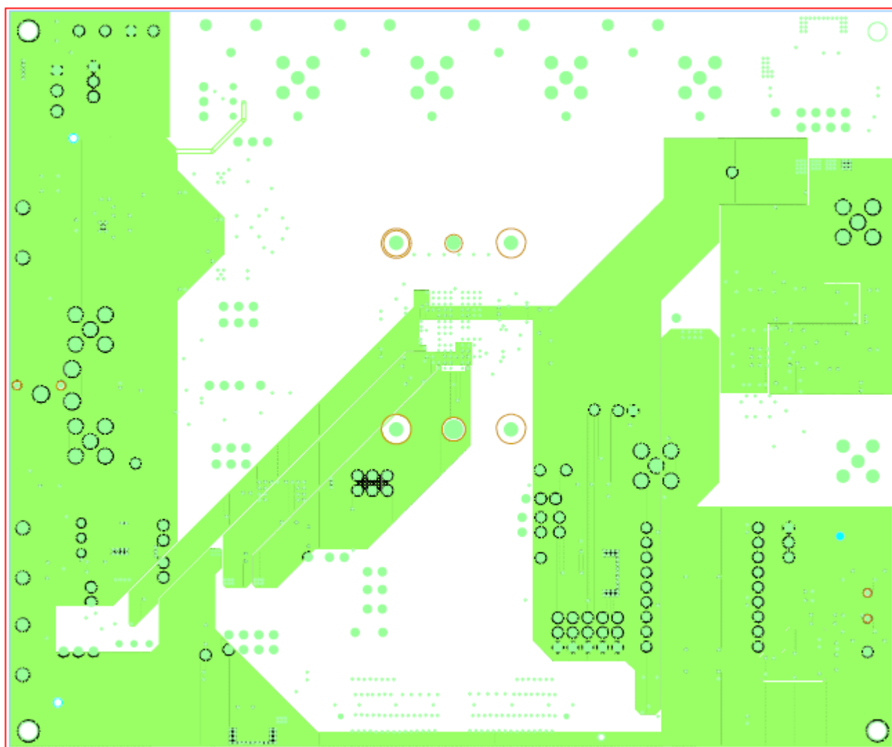
Figure 33. Third Layer - Power
