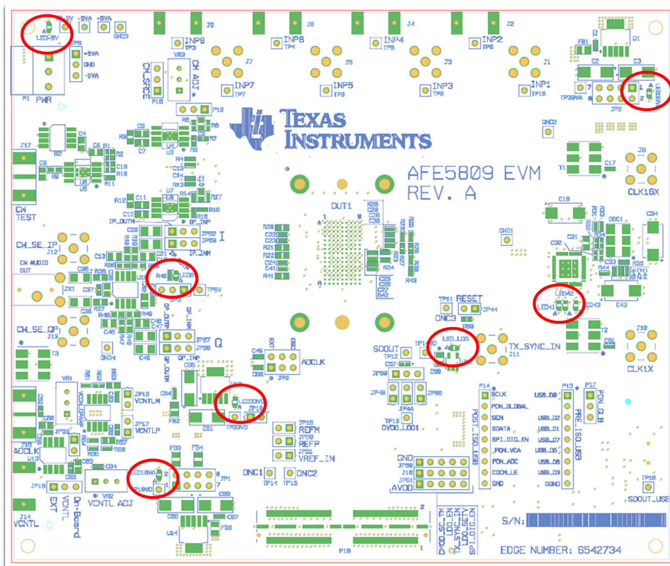
Figure 3. LED Placement
