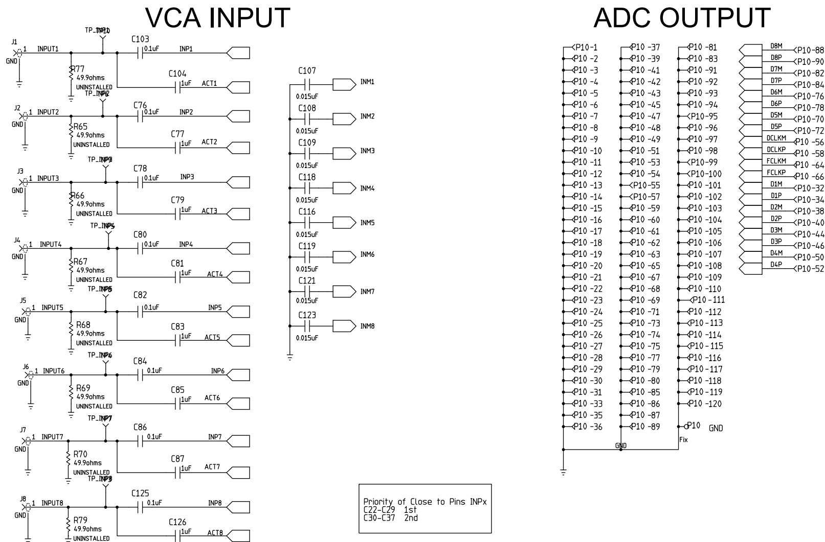
Figure 39. Schematic (Sheet 3 of 10)
