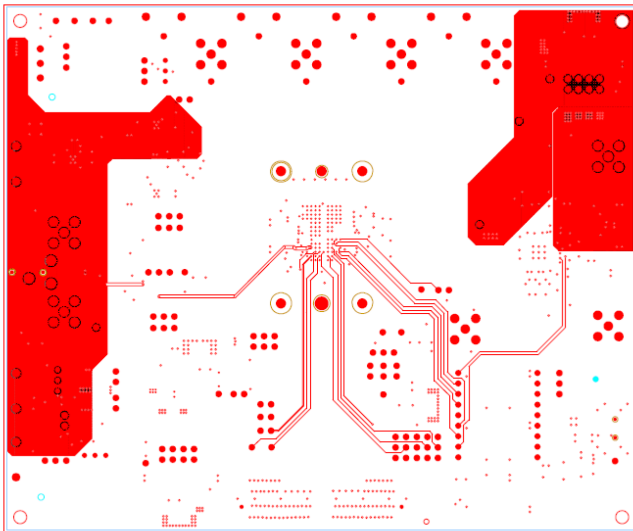
Figure 34. Fourth Layer - Signal
