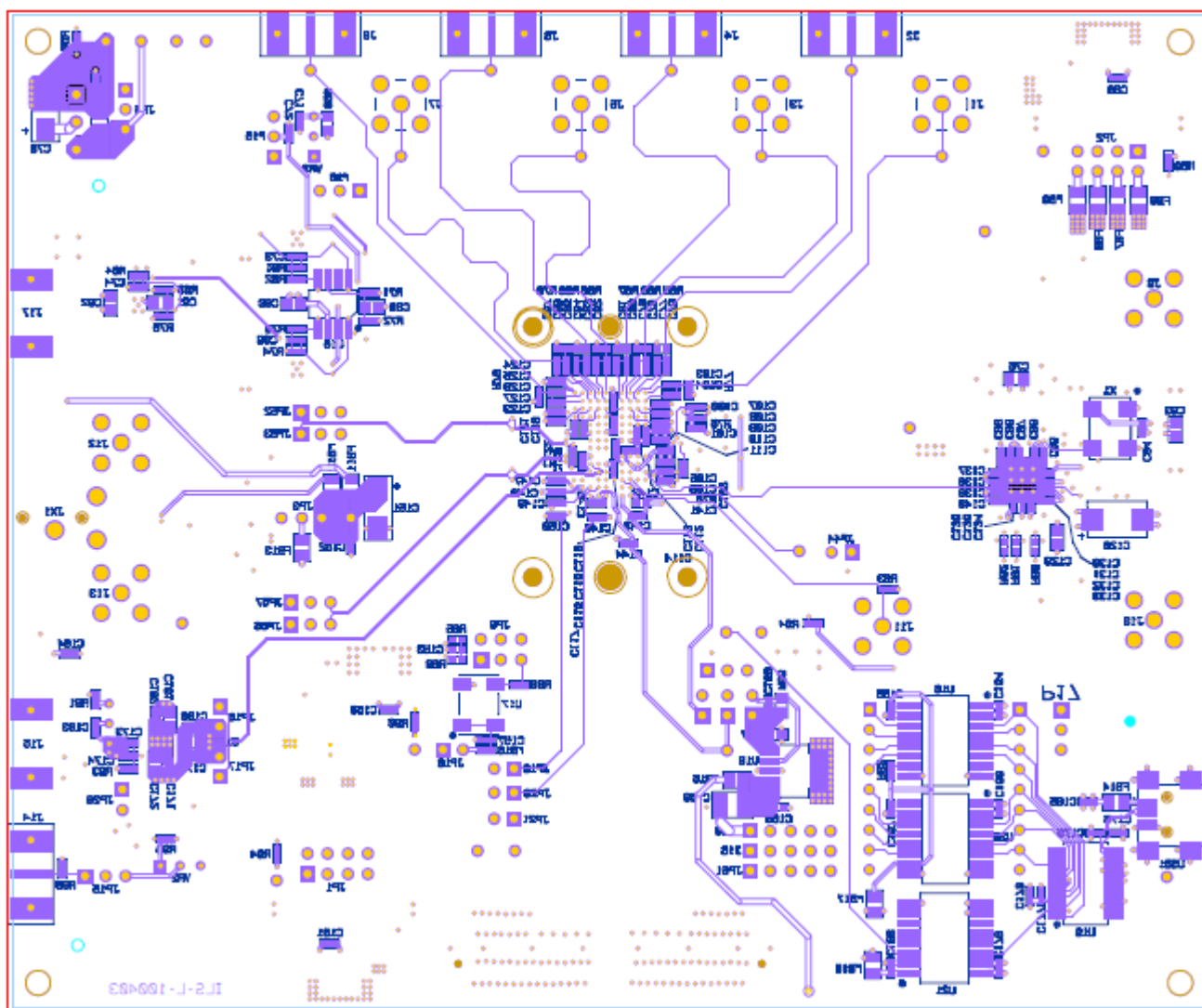
Figure 36. Bottom Layer - Signal
