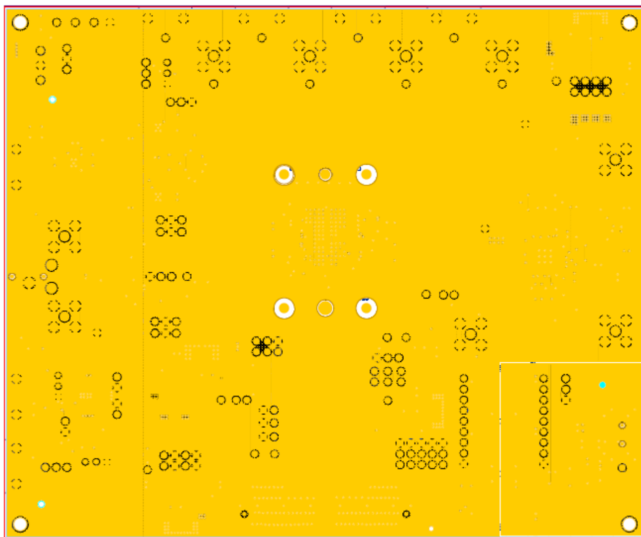
Figure 35. Fifth Layer - Ground
