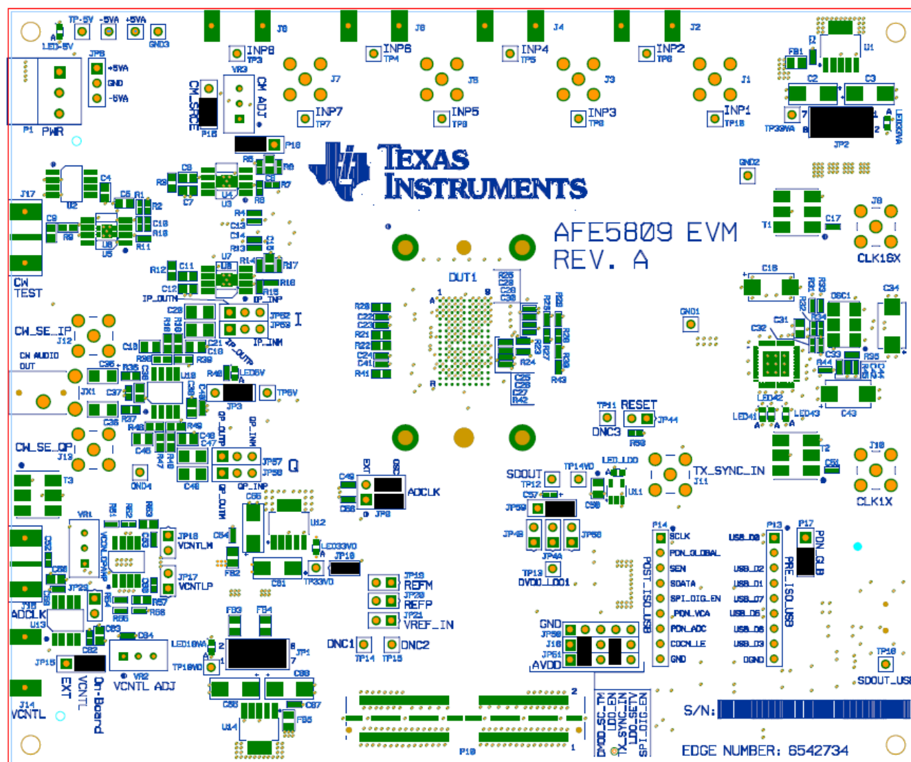
Figure 27. AFE5809EVM Jumper Locations
