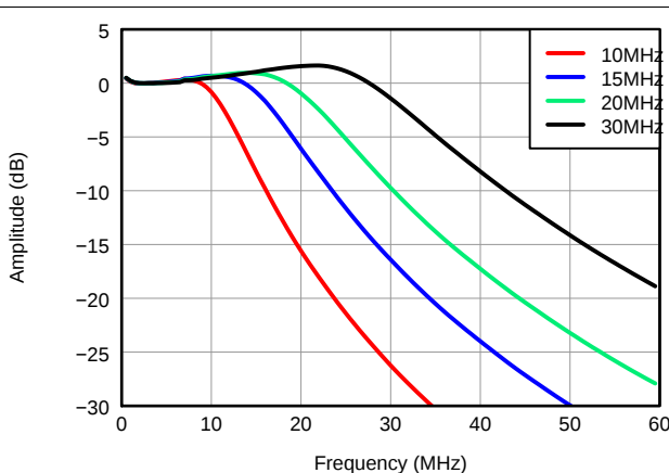
Figure 12. LPF Response
