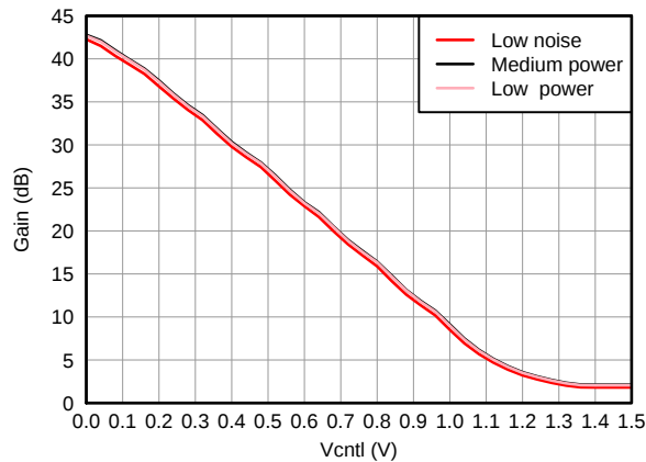
Figure 2. Gain vs V_{\text{CNTL}} , LNA = 18 dB and PGA = 24 dB
