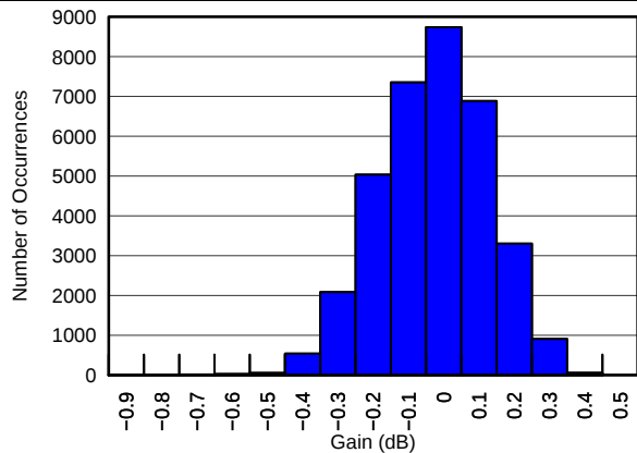
Figure 4. Gain Matching Histogram, V_{\text{CNTL}} = 0.3 V (34951 Channels)
