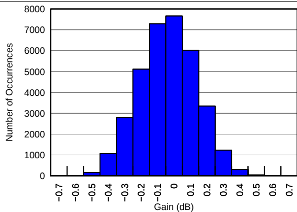
Figure 6. Gain Matching Histogram, V_{\text{CNTL}} = 0.9 V (34951 Channels)
