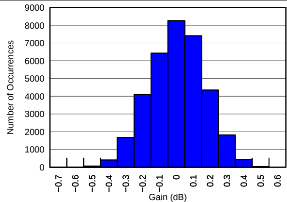
Figure 5. Gain Matching Histogram, V_{\text{CNTL}} = 0.6 V (34951 Channels)
