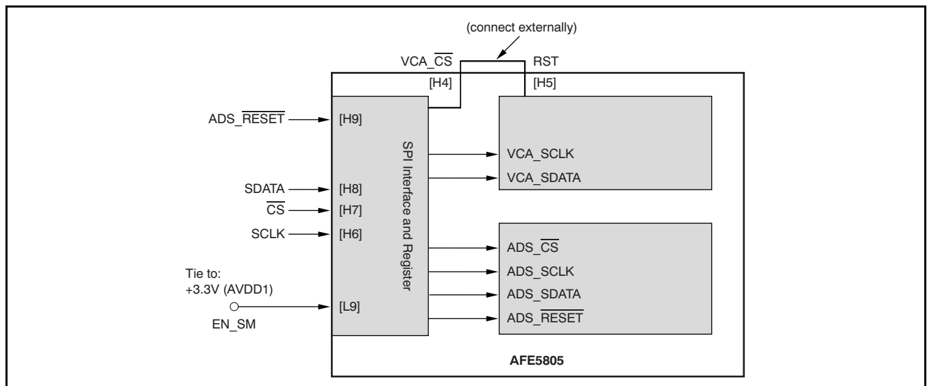
Figure 41. Typical Connection Diagram for the SPI Control Lines
