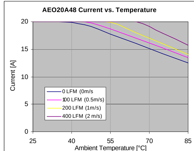
Figure 26. Output Current vs. Temperature for baseplate version at V_{IN} = 48Vdc ( T_J \leq 120^\circ C ).
