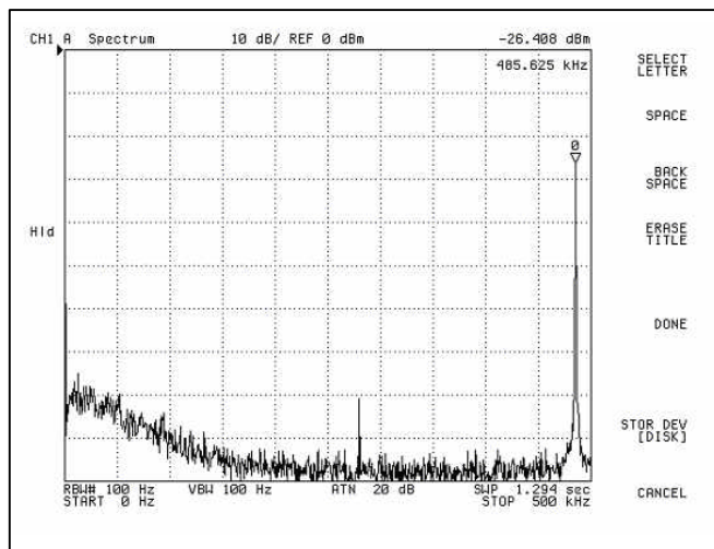
Figure 27. Typical output frequency spectrum (0 – 500kHz) at V_{IN} = 48Vdc , I_O = 50\% Load, C_{OUT} = 0 .
