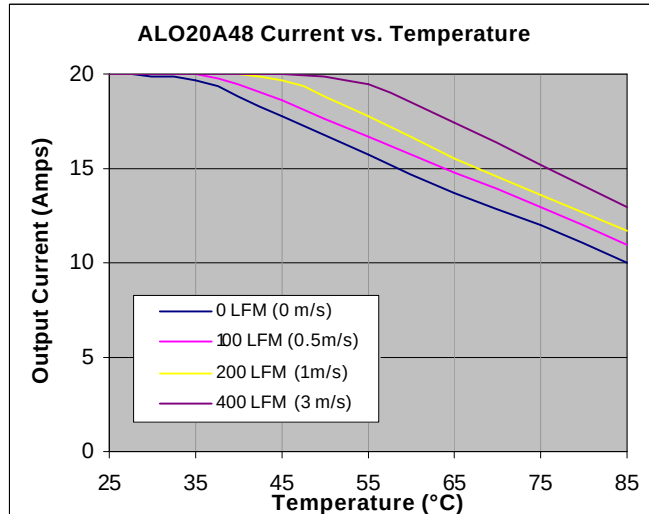
Figure 25. Output Current vs. Temperature for open frame version at V_{IN} = 48Vdc ( T_J \leq 120^\circ C ).
