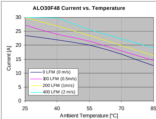
Figure 37. Output Current vs. Temperature for open frame version at V_{IN} = 48Vdc ( T_J \leq 120^\circ C ).
