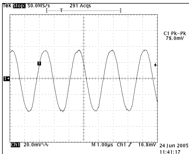
Figure 10. 12V output ripple at V_{IN} = 48\text{Vdc} , I_O = \text{Full Load} , T_A = 25\text{ }^{\circ}\text{C} .
