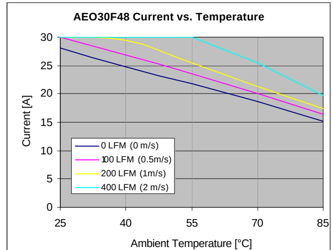
Figure 38. Output Current vs. Temperature for baseplate version at V_{IN} = 48Vdc ( T_J \leq 120^\circ C ).
