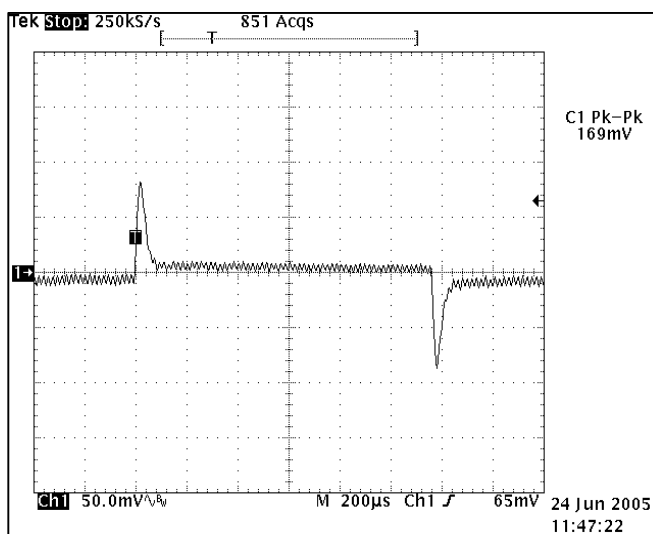
Figure 12. 12V output transient response 50% to 75% step change at V_{IN} = 48\text{Vdc} , T_A = 25\text{ }^{\circ}\text{C} , C_O = 0 .
