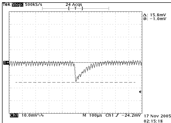
Figure 59. Output transient response at 50% to 75% step, V_{IN} = 48V , T_A = 25^\circ C , C_O = 0 .
