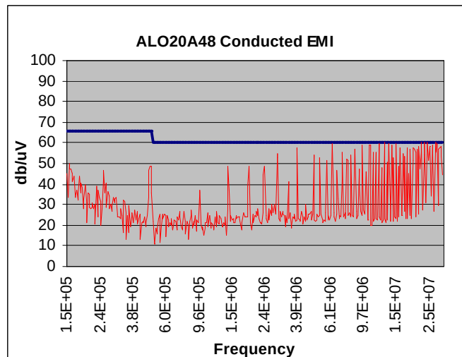
Figure 28. 5V Open frame Conducted EMI per Filter defined in Fig 89. V_{IN} = 48Vdc , I_O = 50\% Resistive Load, T_A = 25^\circ C .
