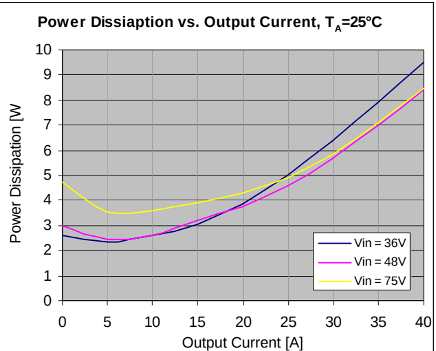
Figure 78. Power Dissipation vs. Load Current at min, nominal and high line, T_A = 25^\circ\text{C} .
