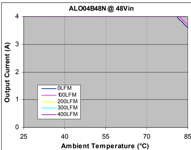
Figure 11. Output Current vs. Temperature for open frame version at V_{IN} = 48V_{dc} , T_A = 25^\circ\text{C} .
