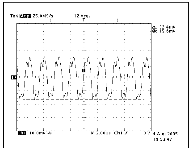
Figure 32. 2.5V OUT Ripple Waveform at V_{IN} = 48Vdc, I_O = Full Load, T_A = 25°C.
