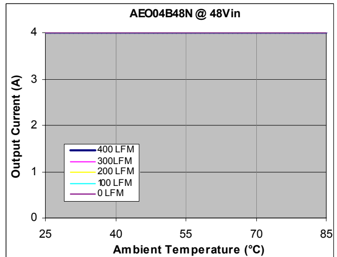
Figure 12. Output Current vs. Temperature for baseplate version at V_{IN} = 48V_{dc} , T_A = 25^\circ\text{C} .
