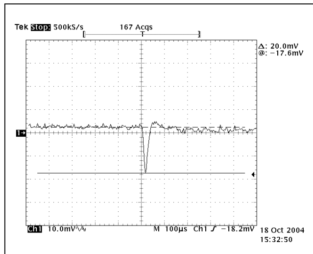
Figure 18. Transient Response at T_A = 25^\circ\text{C} , 5V_{\text{OUT}} Deviation (Lo-Hi).
