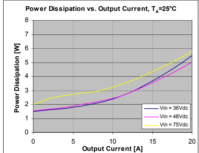
Figure 30. Power Dissipation vs. Load Current at I_O = Full Load, T_A = 25°C (ambient temperature).
